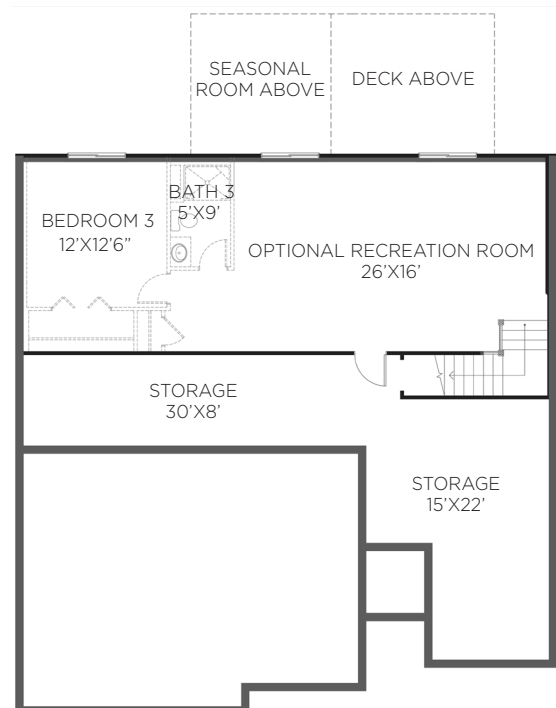
BASEMENT LEVEL
