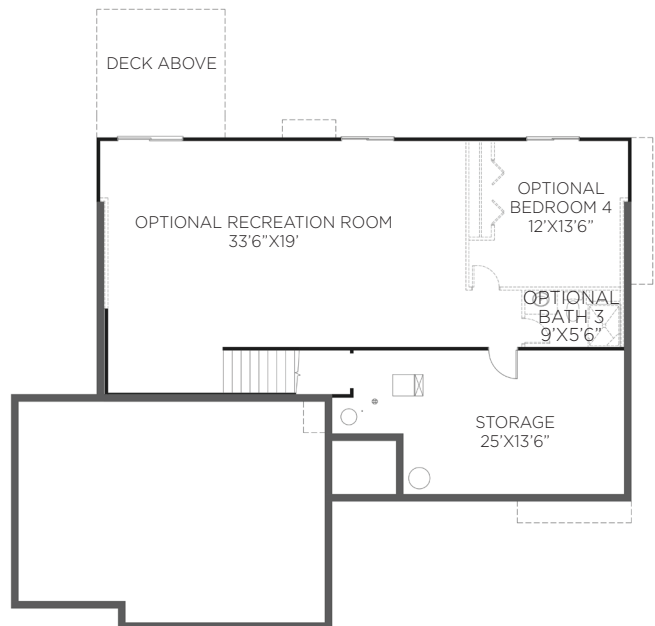
BASEMENT LEVEL
