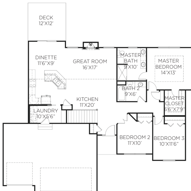
MAIN LEVEL
